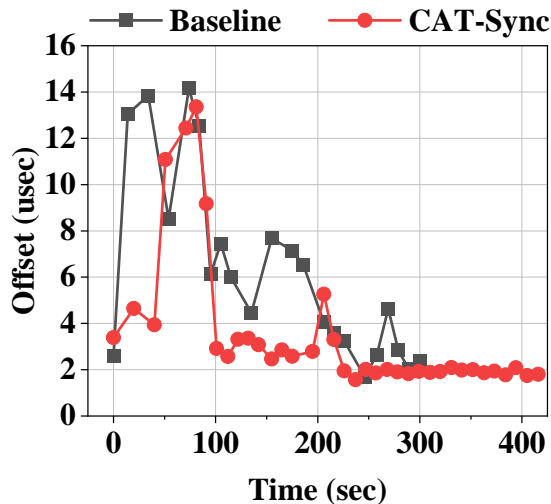
Fig. 3. Clock offset for long-term synchronization.
